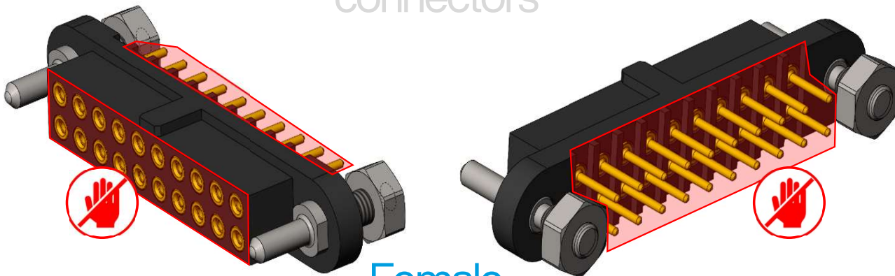
Female connectors
