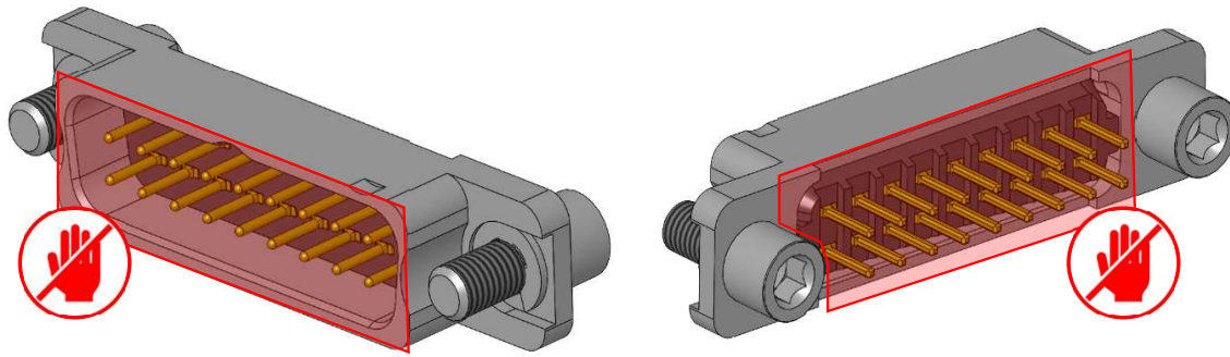
Male connectors
