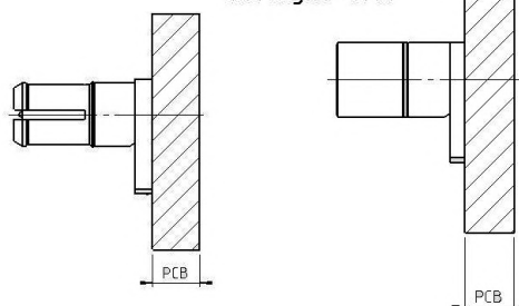
Straight SMT
