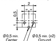
HF 30-2400-xx PCB lay-out
