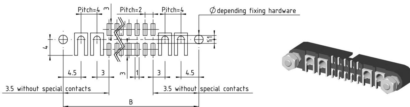
PCB layout for CMM220 male series
