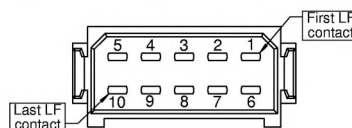
Male connectors ( shown looking onto mating face )
