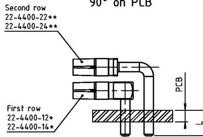
90° on PCB
