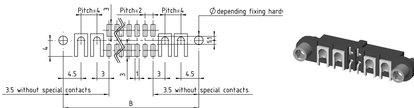
PCB layout for CMM220 female series
