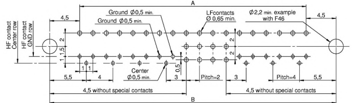
PCB layout for CMM320 series ( Shown looking onto mating face )
