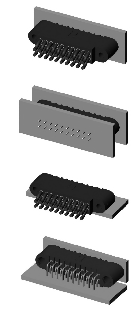
Female connectors ( shown looking onto mating face )
