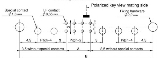
PCB layout CMM220 series
