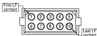
Female connectors ( shown looking onto mating face )
