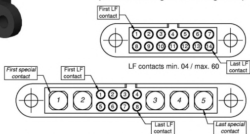
Female connectors ( shown looking onto mating face )
