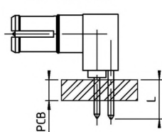
90° on PCB
