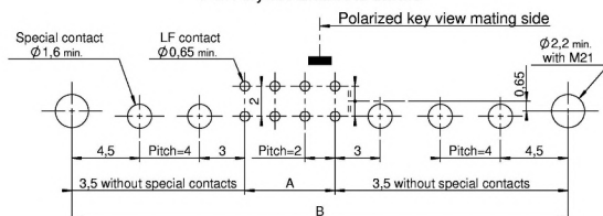
PCB layout CMM220 series
