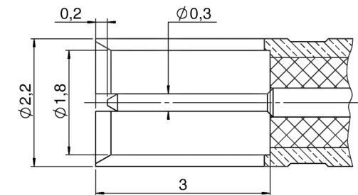
HF female contact insertion
