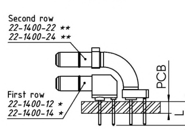
90° on PCB
