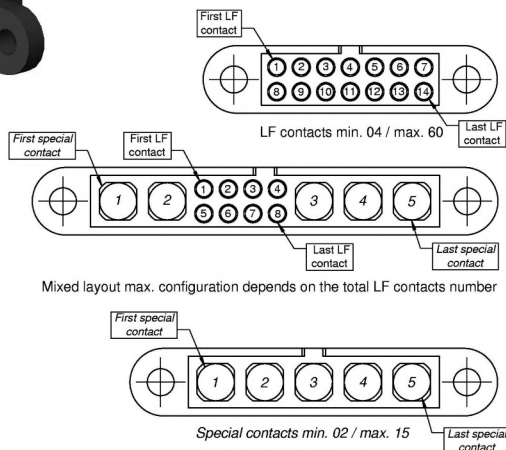
Female connectors ( shown looking onto mating face )
