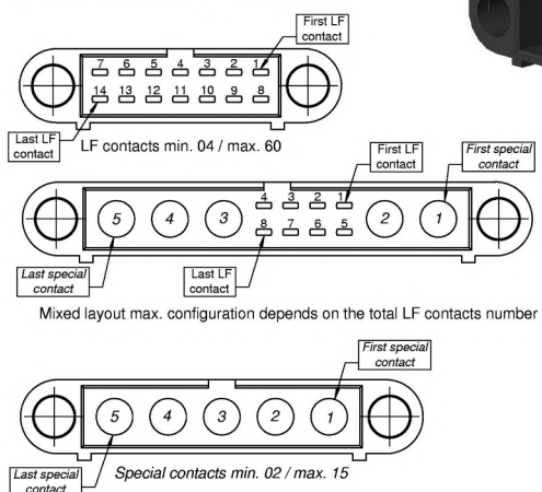
Male connectors ( shown looking onto mating face )
